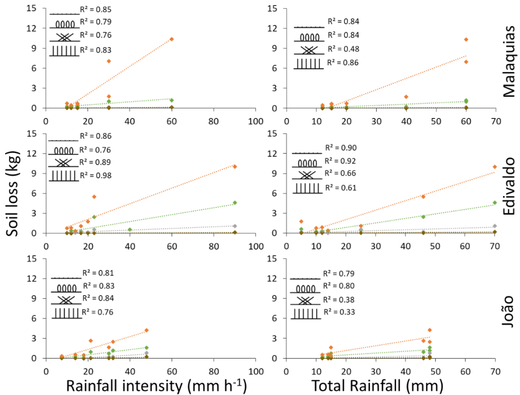
Figure 7. Soil loss as a function of rainfall volume and intensity, for all sites and plots.
